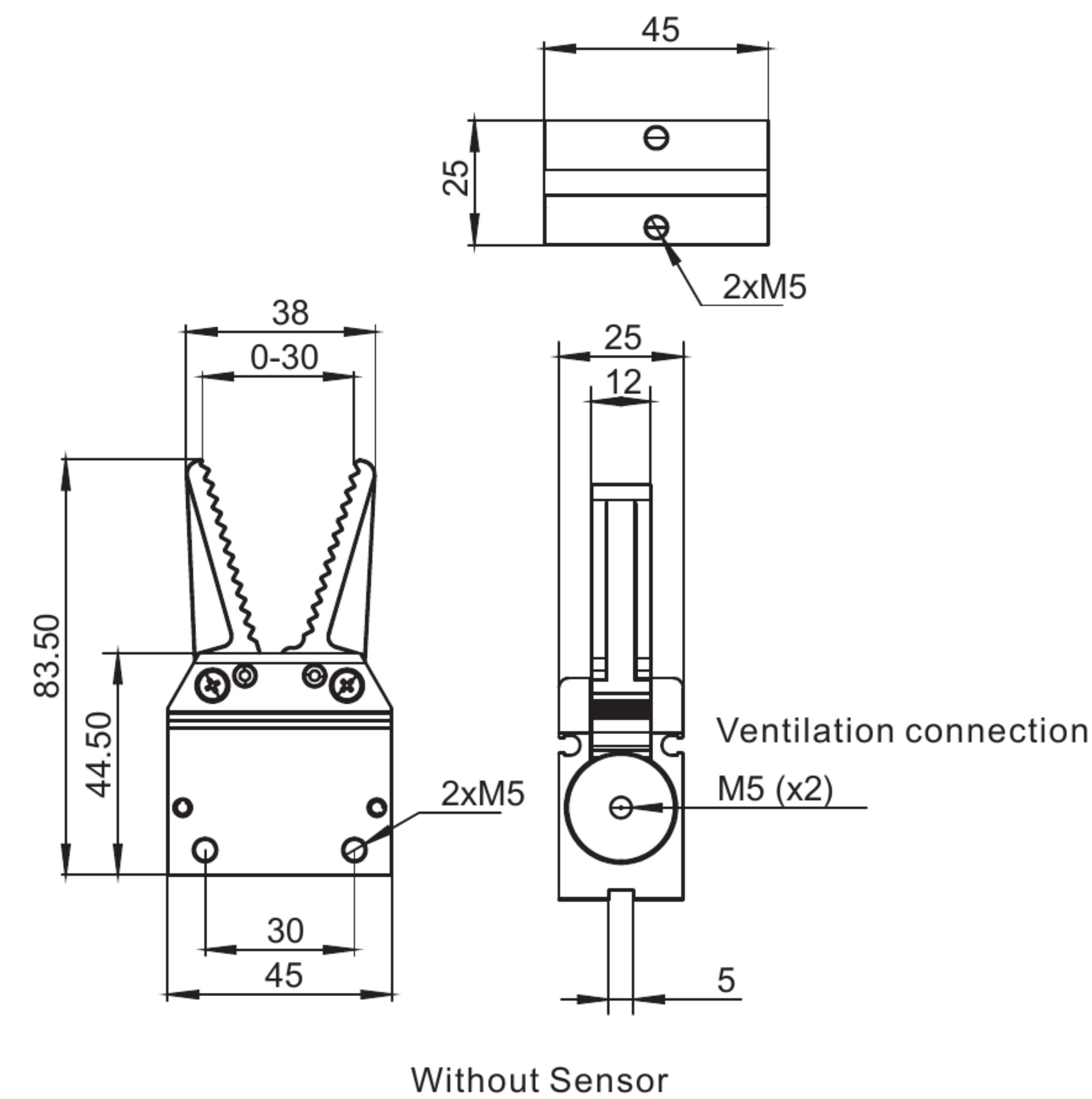
GRA20A Without Sensor
