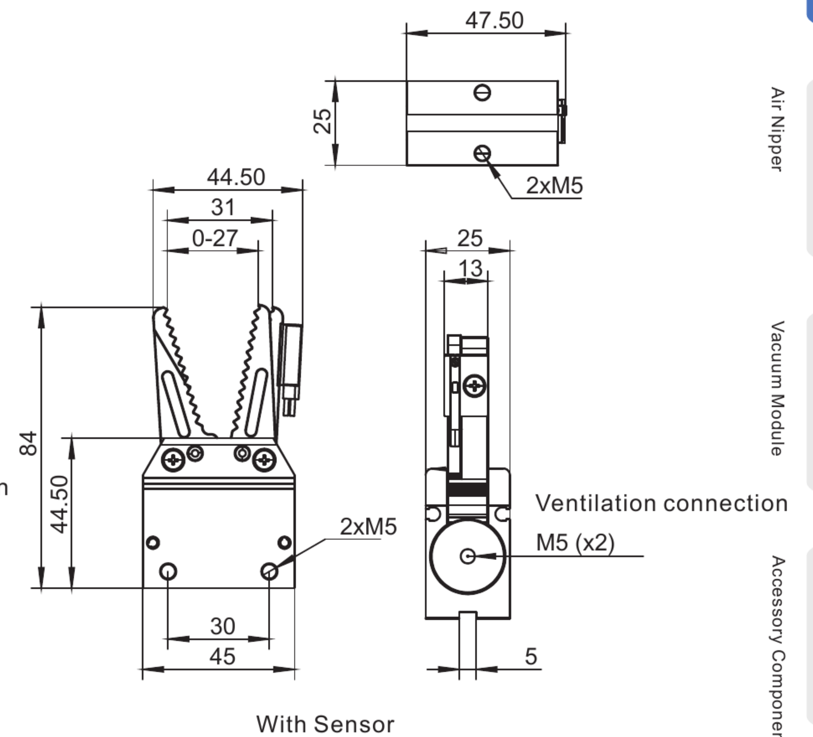
GRA20A-CN(CP) With Sensor
