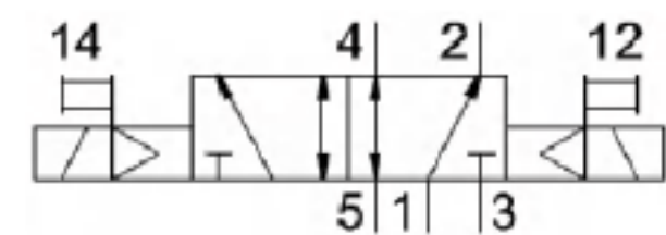
B52 Two-position double electronic control
