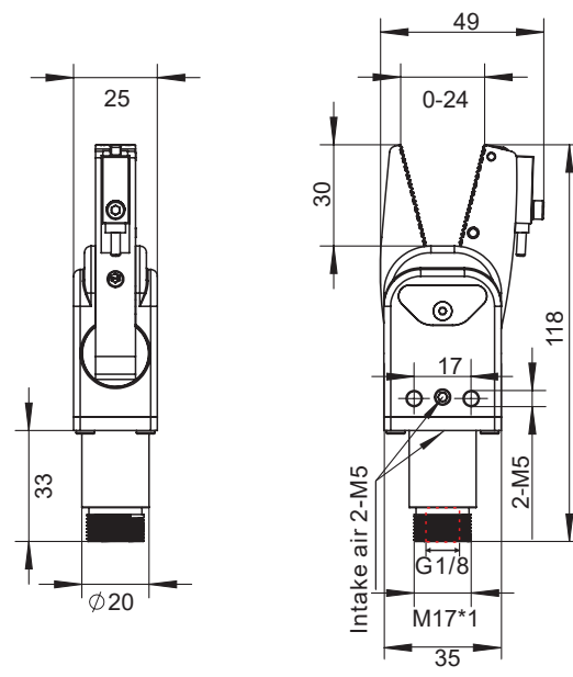
With Sensor
