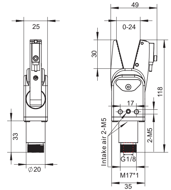
With Sensor
