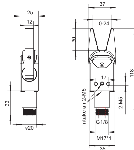
Without Sensor
