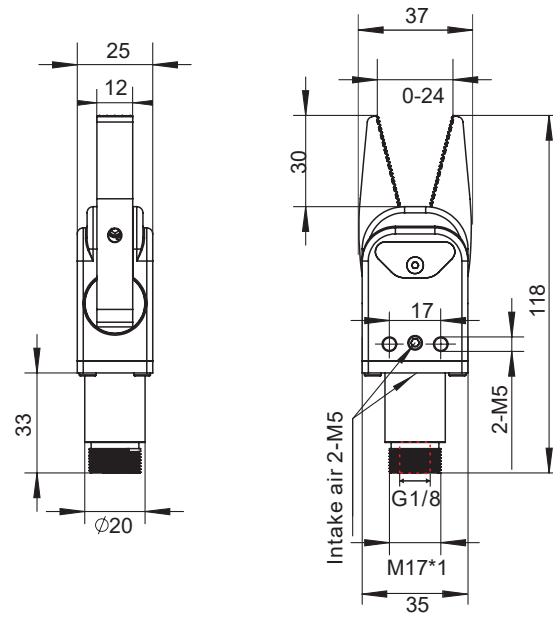
Without Sensor
